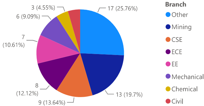
Branch Distribution
